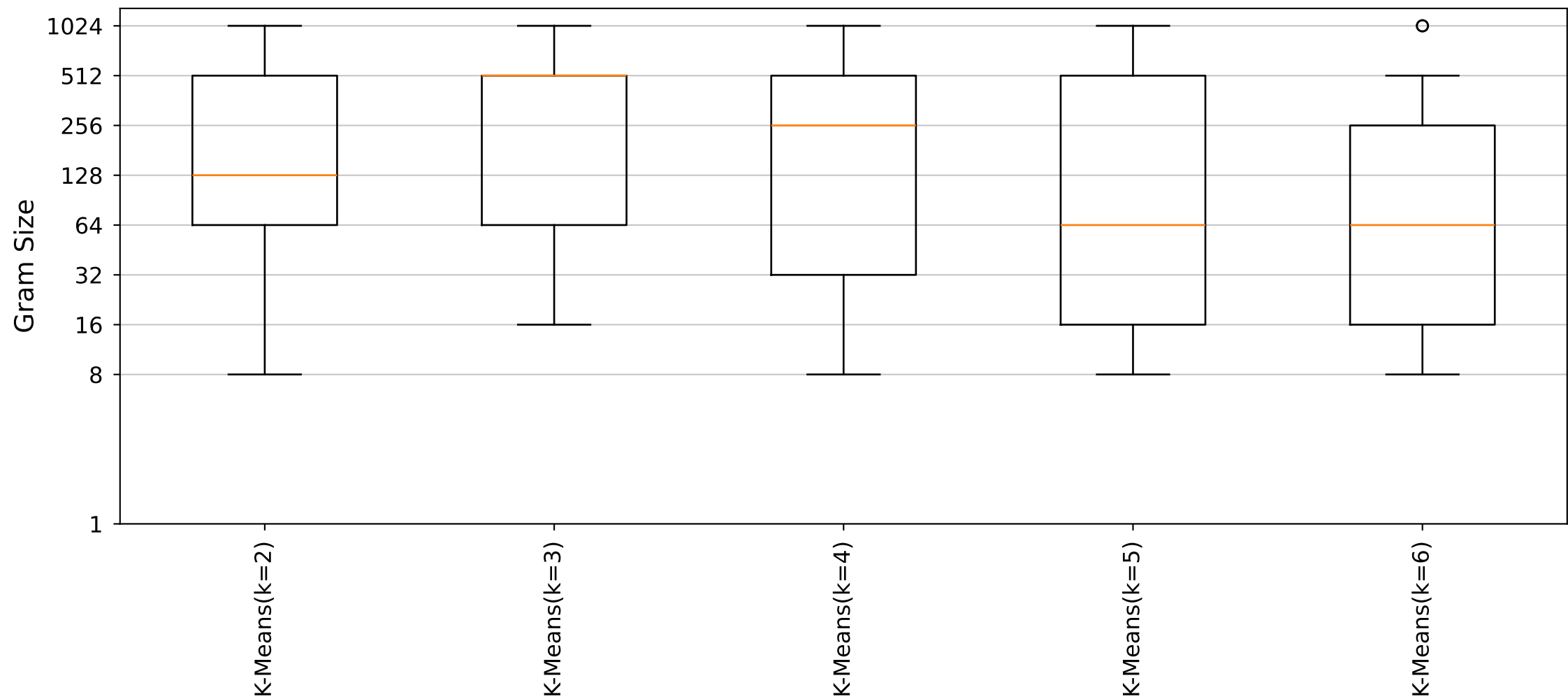
YARA Rules Gram Size Distribution (Cluster24_Size6 dataset)
